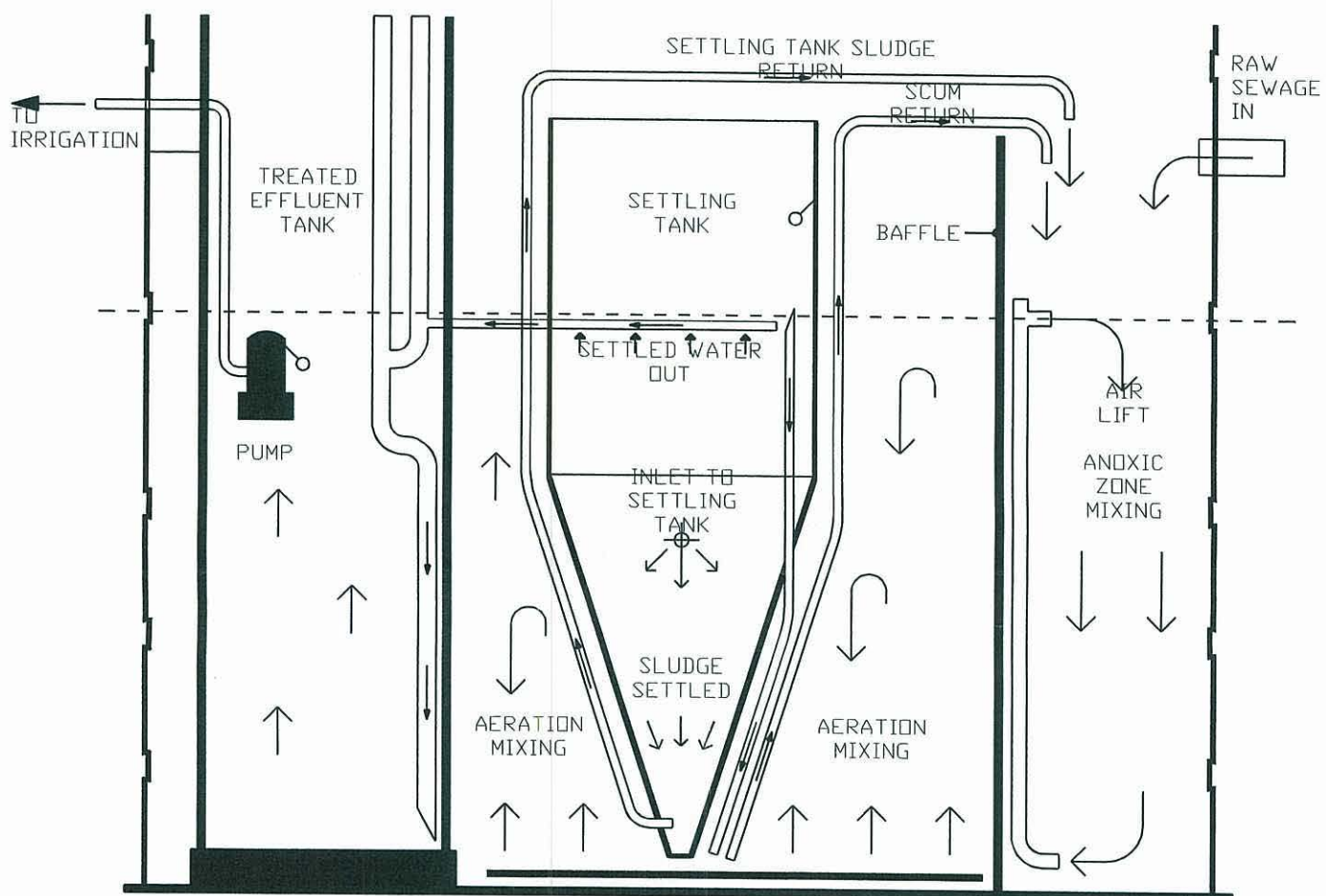
TREATMENT TANK FLOW SCHEMATIC NOT TO SCALE
